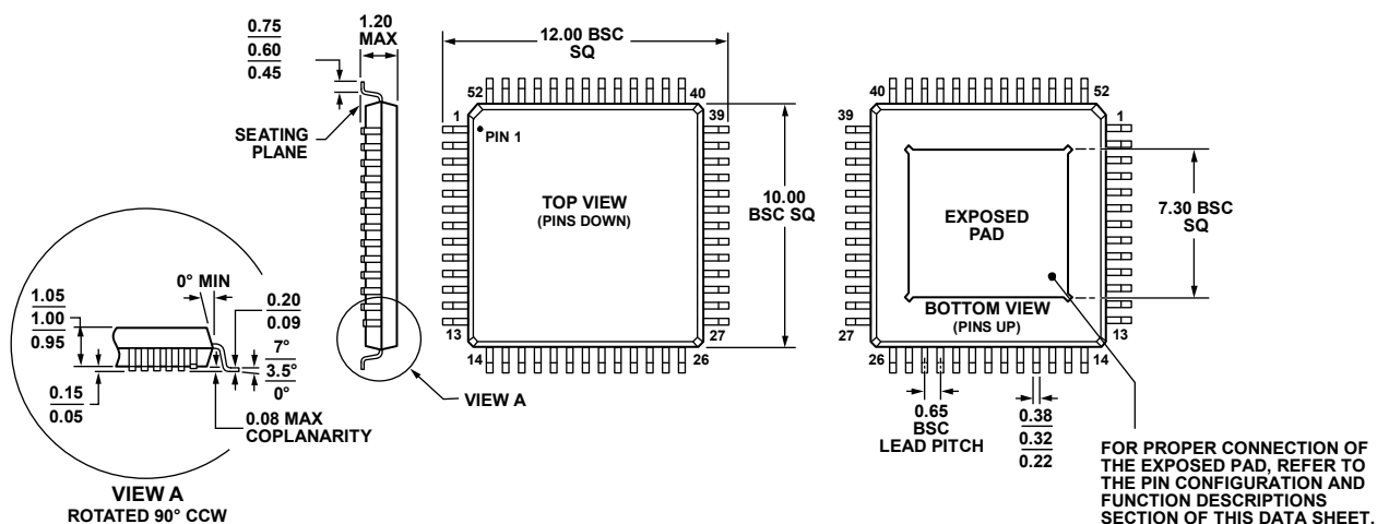
Figure 33. 52-Lead Thin Quad Flat Package, Exposed Pad [TQFP_EP] (SV-52-2) Dimensions shown in millimeters
