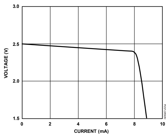
Figure 20. Voltage Reference Output vs. Current Load
