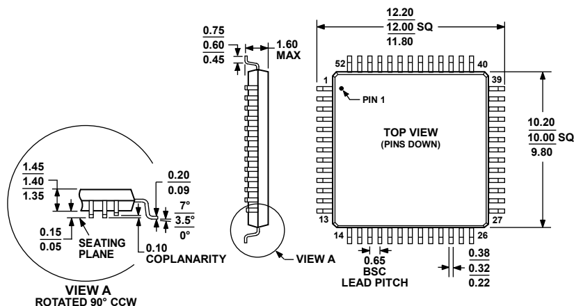
Figure 32. 52-Lead Low Profile Quad Flat Package [LQFP] (ST-52) Dimensions shown in millimeters
