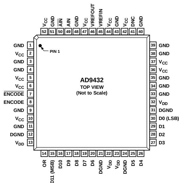
Figure 3. Pin Configuration, LQFP
