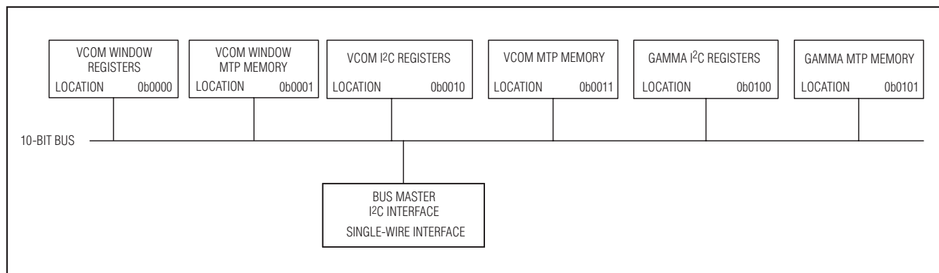
Figure 3. 10-Bit Bus
