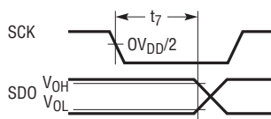
Figure 3. SDO Data Valid Hold after SCK \downarrow
