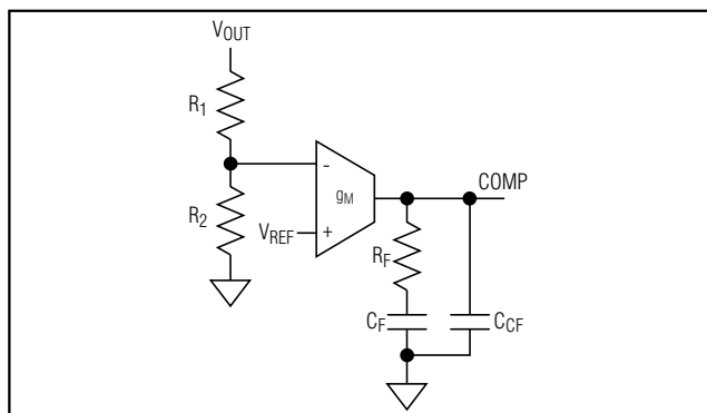
Figure 7. Type II Compensation Network.
