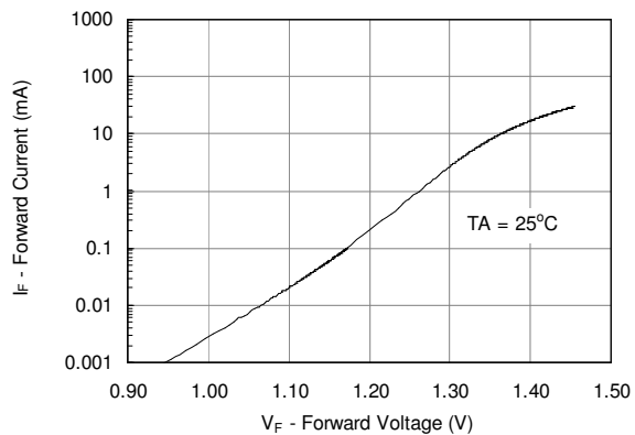
Figure 15: Input Current vs Forward Voltage
