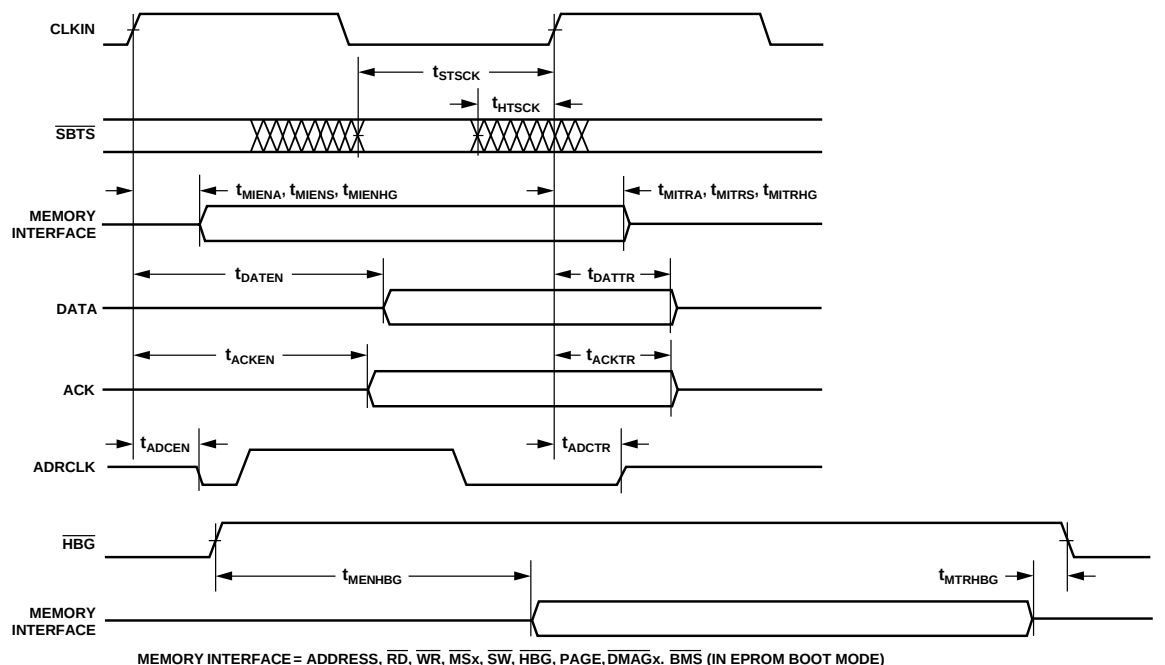
Figure 14. Three-State Timing
