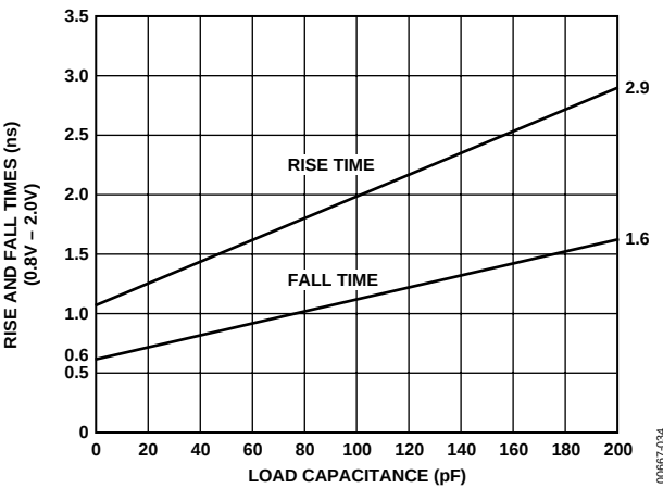
Figure 34. Typical Output Rise Time (0.8 V to 2.0 V) vs. Load Capacitance ( V_{DD} = 5\text{ V} )
