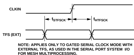
Figure 18. Serial Ports
