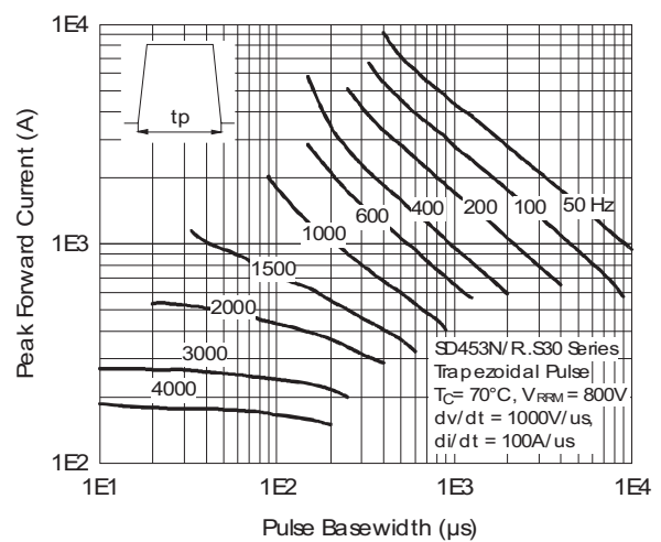
Fig. 35 - Frequency Characteristics
