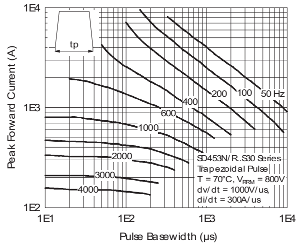
Fig. 33 - Frequency Characteristics
