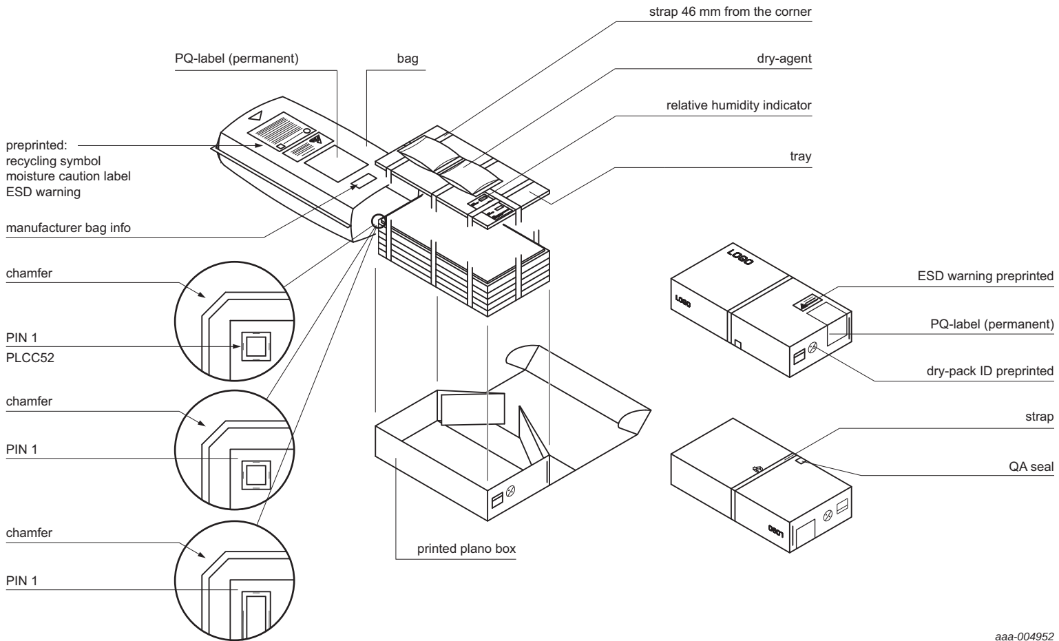
Fig 34. Packing information 5 tray
