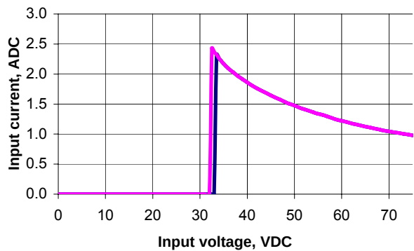
Figure 6. QLS25ZD Input Characteristic
