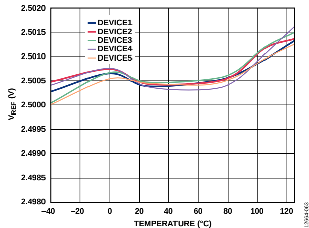
Figure 52. V_{REF} vs. Temperature (B Grade)
