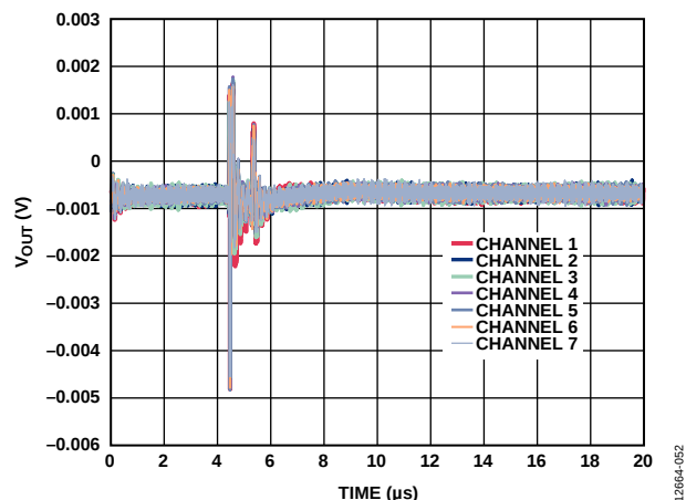
Figure 43. Analog Crosstalk
