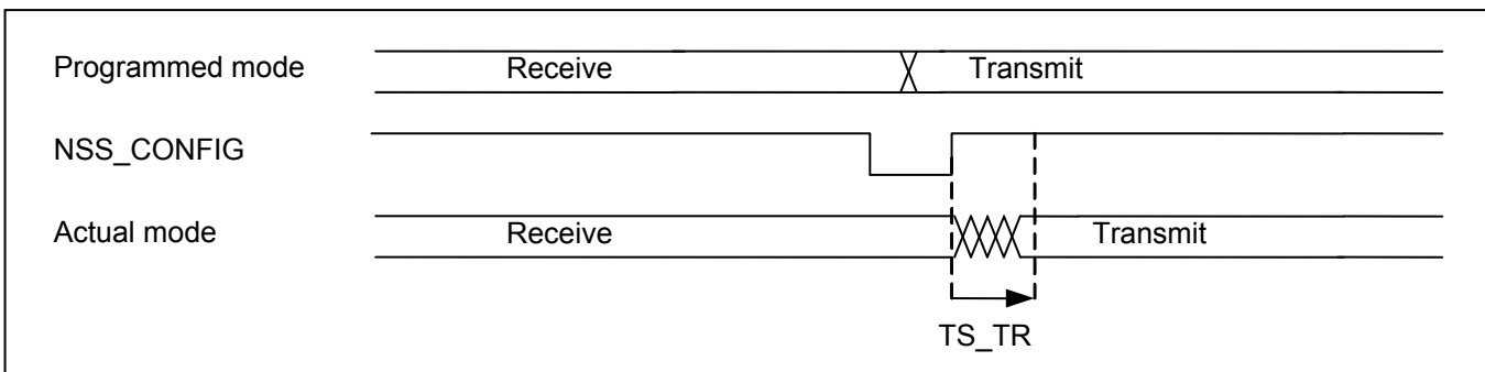
Figure 22: Sequence from receiver to transmitter mode
