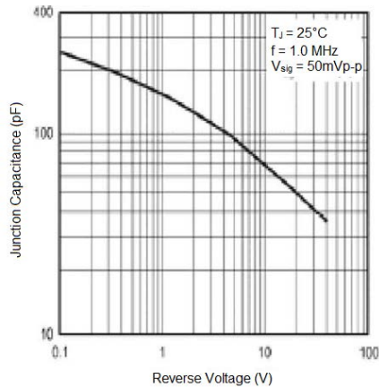
Figure. 5 Typical Junction Capacitance
