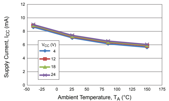
Supply Current (On) versus Temperature
