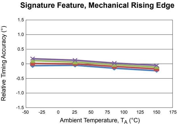
Timing Accuracy versus Ambient Temperature AG = 2.5 mm; relative to T_A = 25^\circ\text{C} , S_{\text{ROT}} = 1000\text{ rpm}
