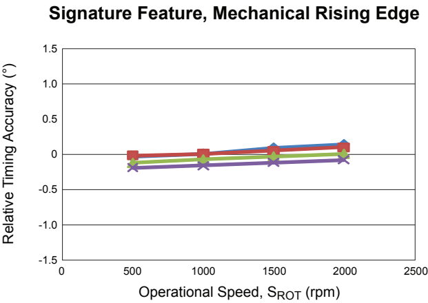
Timing Accuracy versus Operational Speed AG = 0.5 mm; relative to T_A = 25^{\circ}\text{C} , S_{\text{ROT}} = 1000\text{ rpm}
