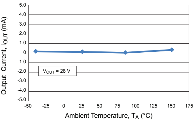
Output Current (Off) versus Temperature
