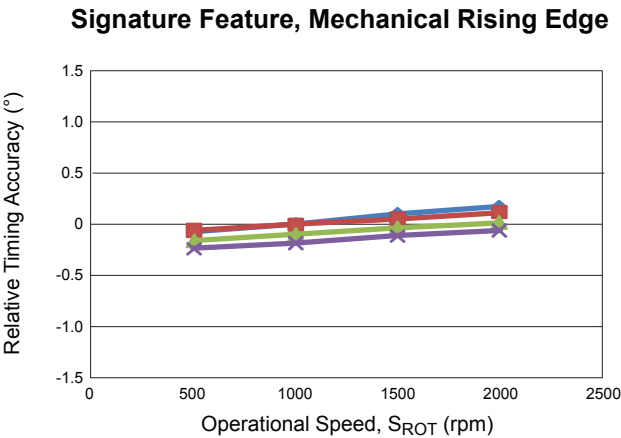
Timing Accuracy versus Operational Speed AG = 2.5 mm; relative to T_A = 25^{\circ}\text{C} , S_{\text{ROT}} = 1000\text{ rpm}
