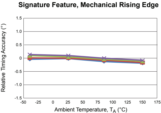
Timing Accuracy versus Ambient Temperature AG = 0.5 mm; relative to T A = 25°C, S ROT = 1000 rpm
