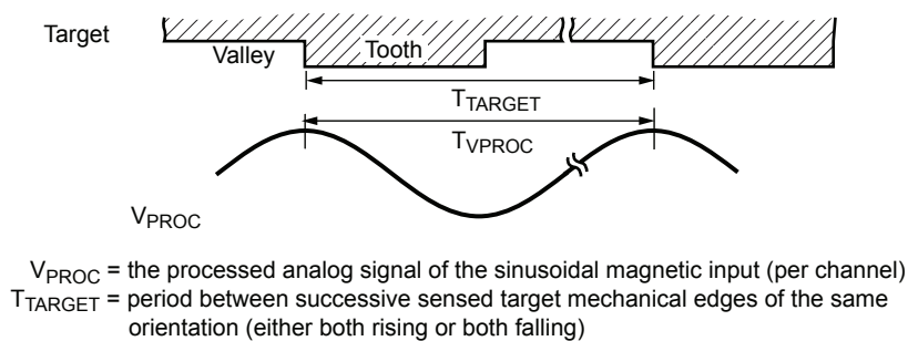
Figure 2. Definition of T_{TARGET}
