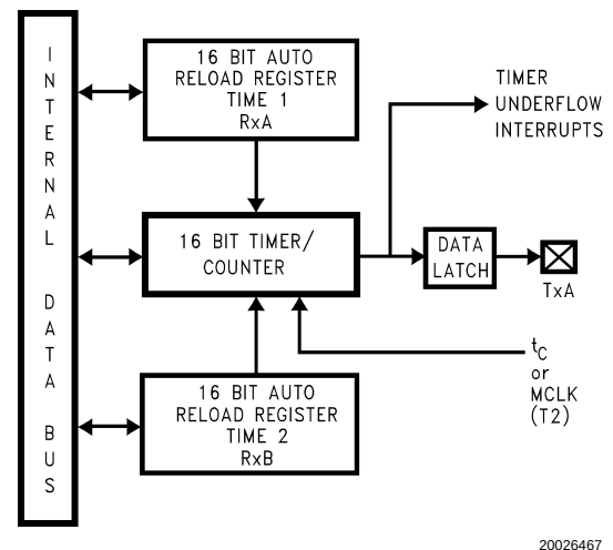
FIGURE 14. Timer in PWM Mode
