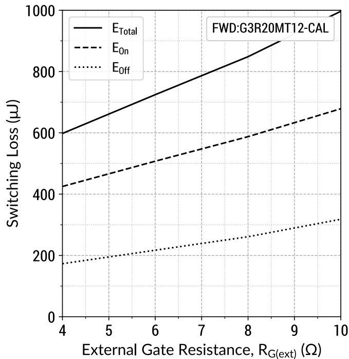
Figure 19: Resistive Switching Energy v/s R_{G(ext)} ( V_{DD} = 800V )
