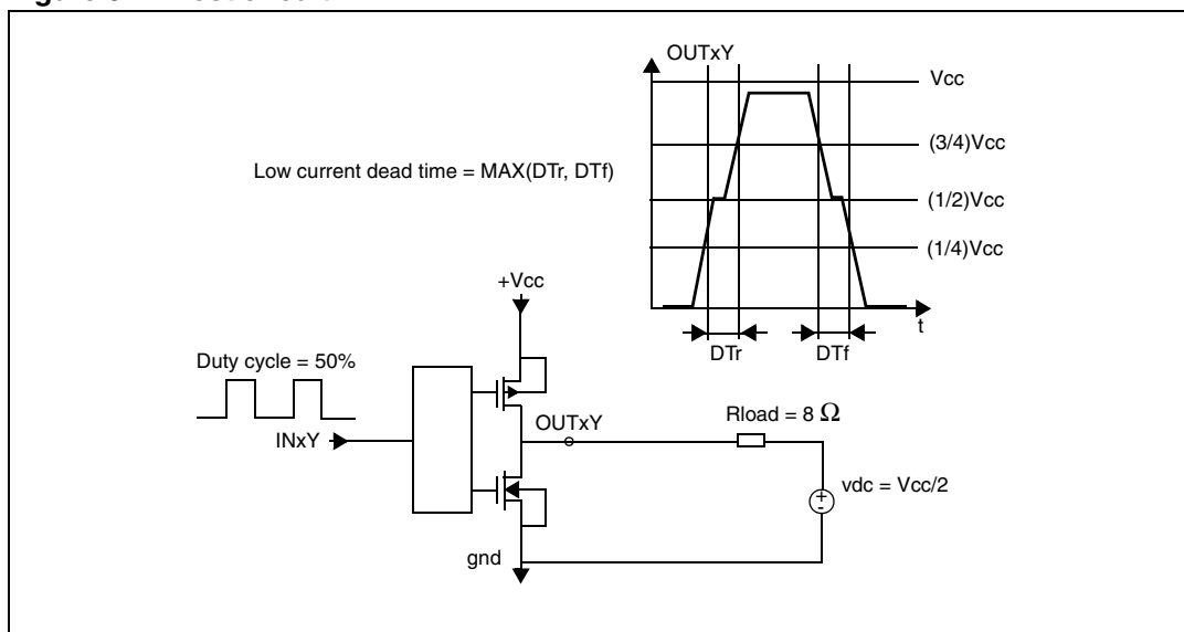
Figure 3. Test circuit
