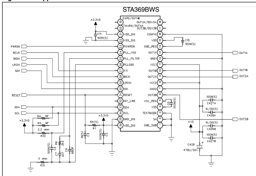
Figure 27. Applications circuit
