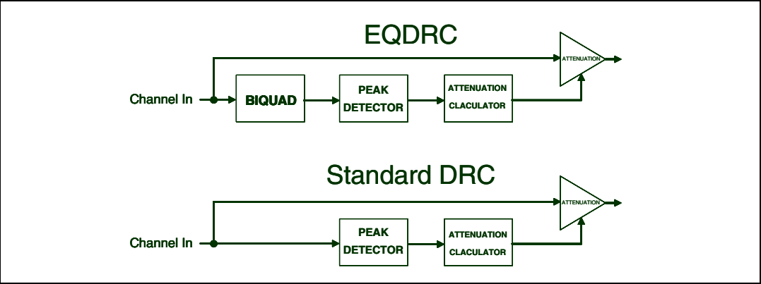
Figure 20. EQDRC scheme
