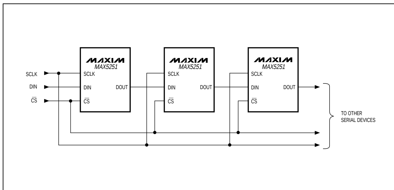
Figure 7. Daisy-Chaining MAX5251s
