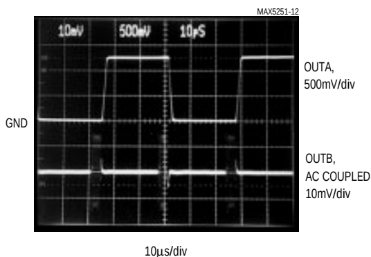
ANALOG CROSSTALK
