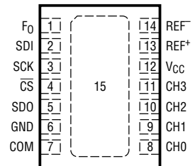
DE PACKAGE 14-LEAD (4mm x 3mm) PLASTIC DFN
