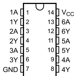
J, W, D, DB, N, NS, or PW Package 14-Pin CDIP, CFP, SOIC, SSOP, SO, or TSSOP Top View
