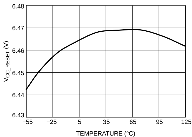
Figure 11. V CC_RESET vs. Temperature
