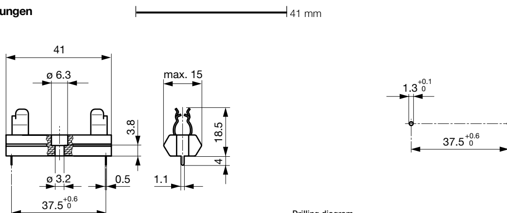
Drilling diagram
