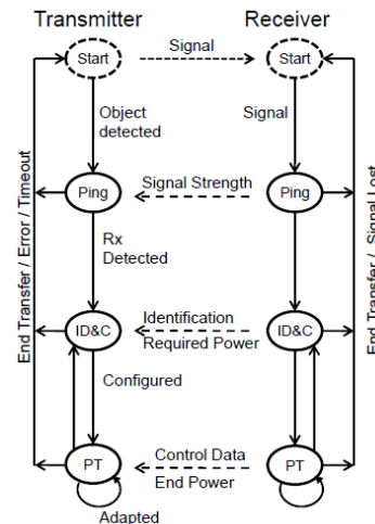
Figure 13. WPC System Feedback control.
