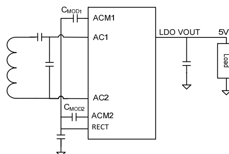
Figure 14. Modulation components.
