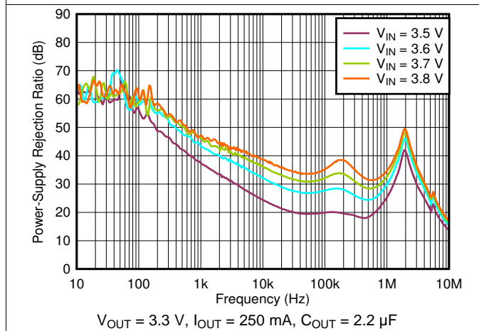
Figure 27. PSRR vs Frequency and V_{IN}
