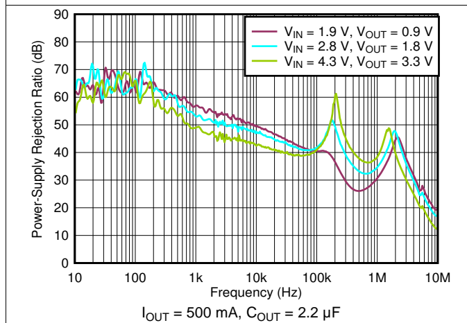
Figure 29. PSRR vs Frequency
