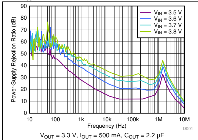
Figure 25. PSRR vs Frequency and V_{IN}
