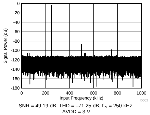
Figure 3. Typical FFT
