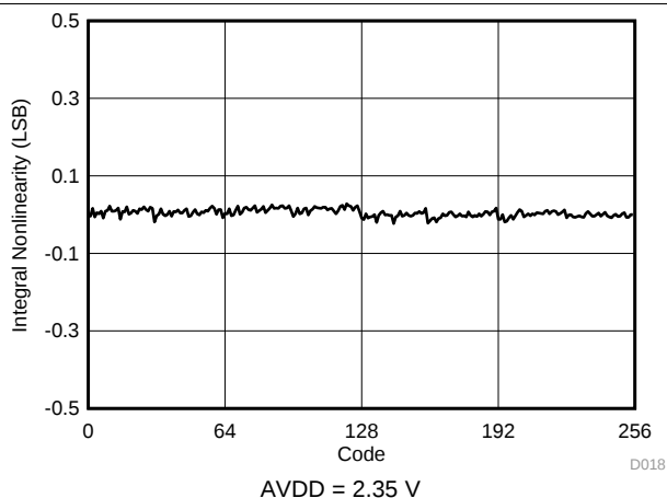
Figure 15. Typical INL
