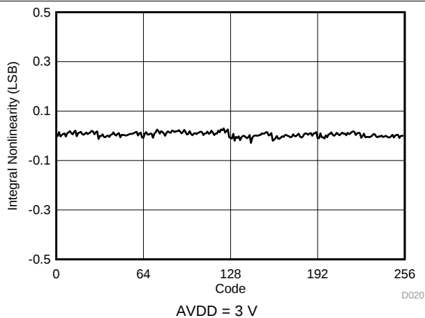
Figure 17. Typical INL
