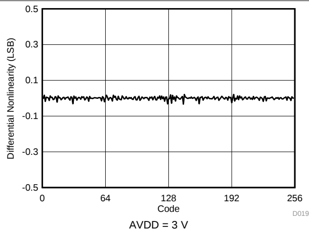
Figure 16. Typical DNL
