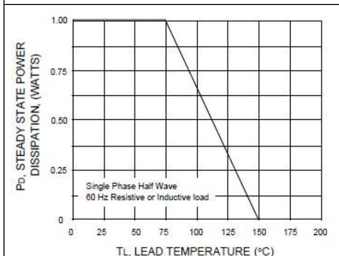
FIG.3 - STEADY STATE POWER DERATING
