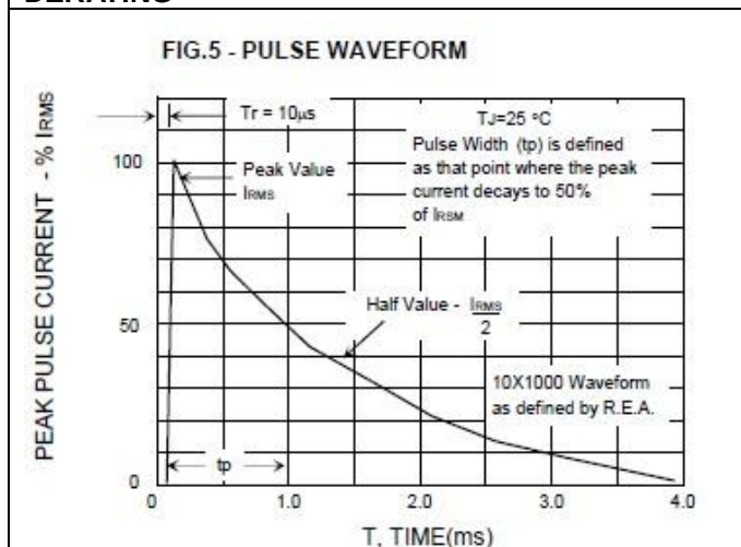
FIG.5 - PULSE WAVEFORM
