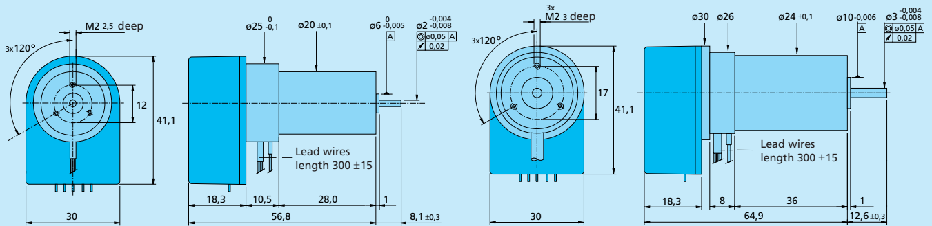
Encoders HEDS 5500, 5540 with Brushless DC-Servomotor 2036 U ... B K312
