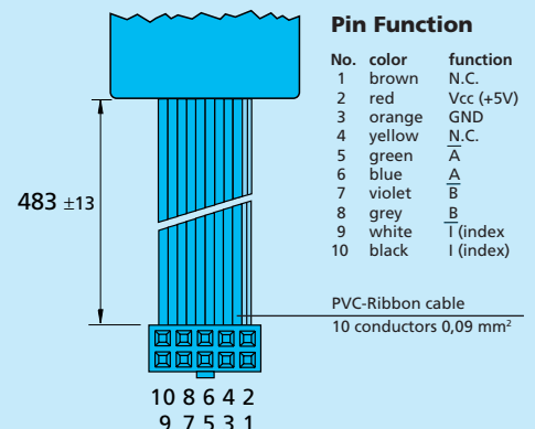
Connector DIN-41651 grid 2,54 mm
