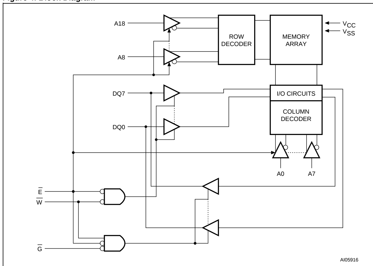
Figure 4. Block Diagram
