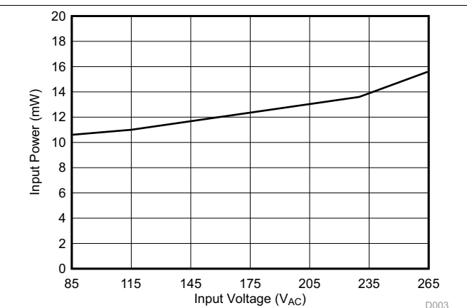
Figure 24. No Load Power Consumption
