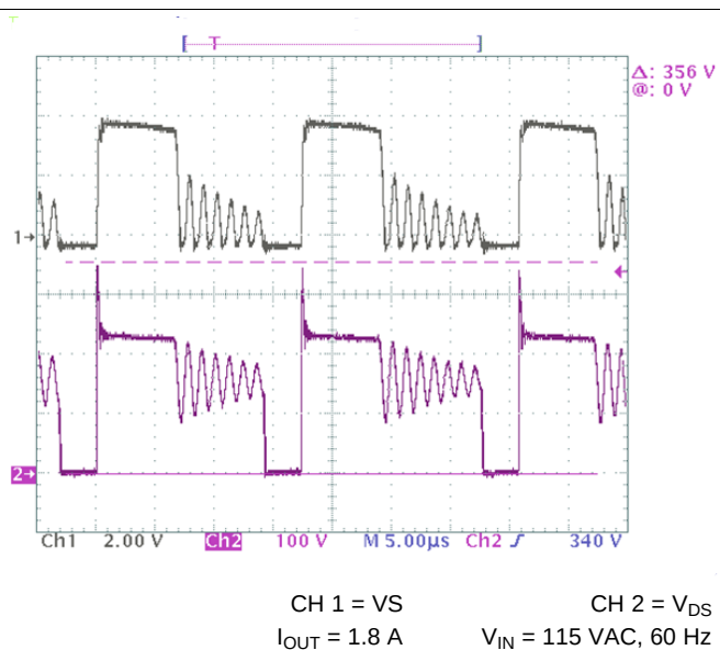
Figure 20. Switching Waveform
