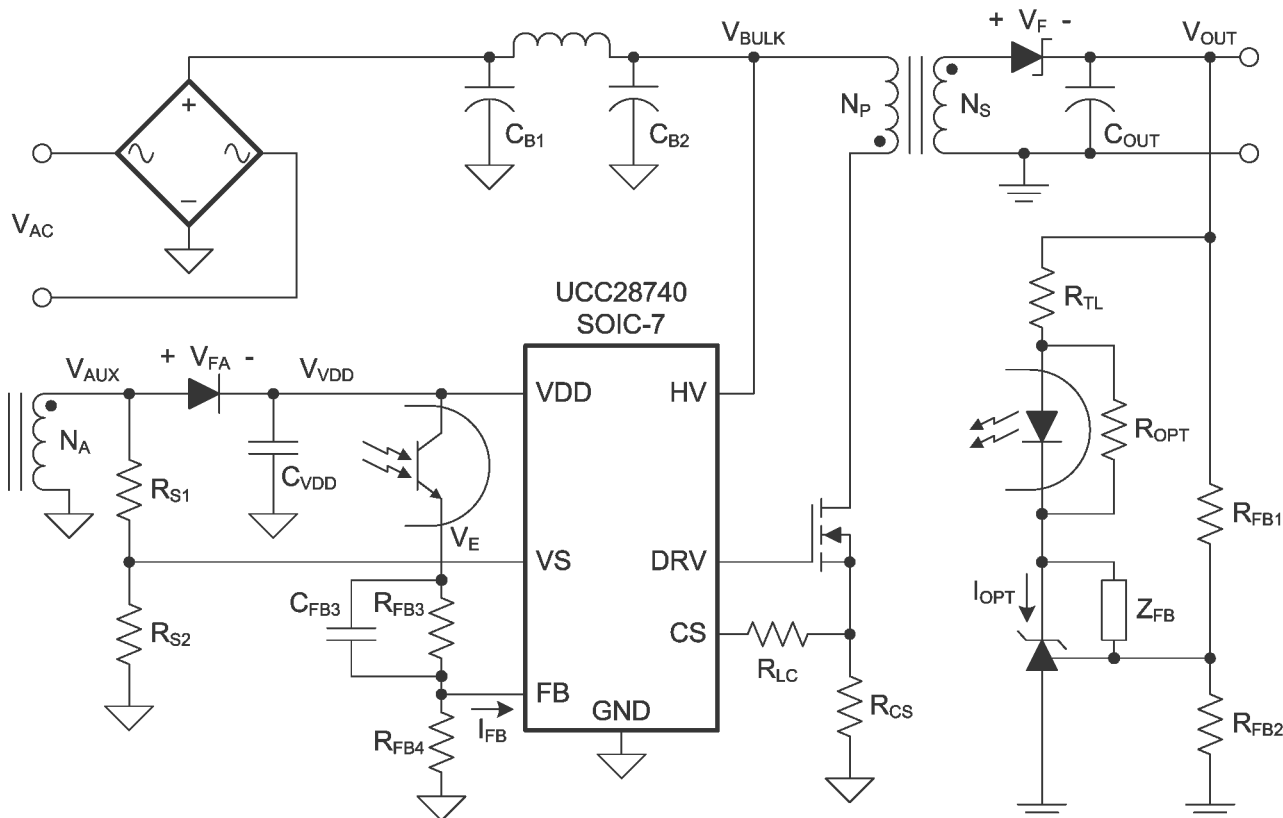
Figure 18. Design Procedure Application Example
