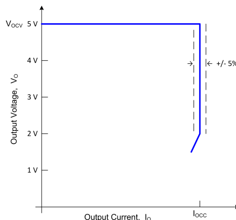
Typical V-I Diagram
