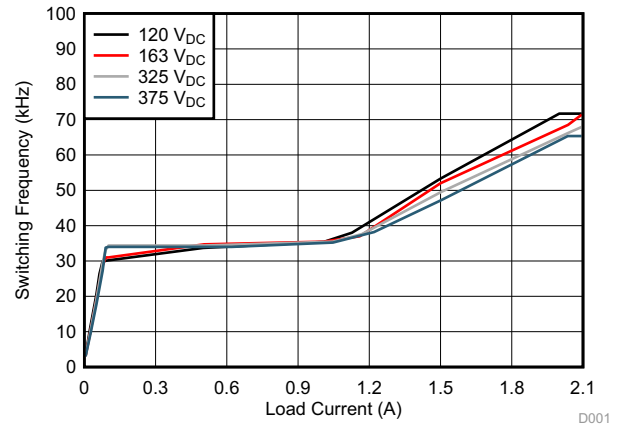
Figure 26. Control Law
