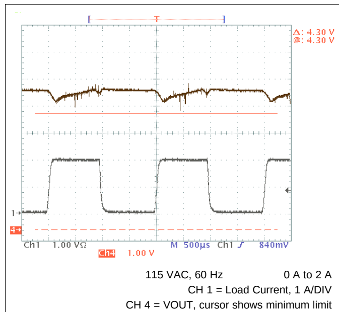
Figure 19. Transient Response
