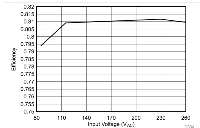
Figure 23. Average Efficiency
