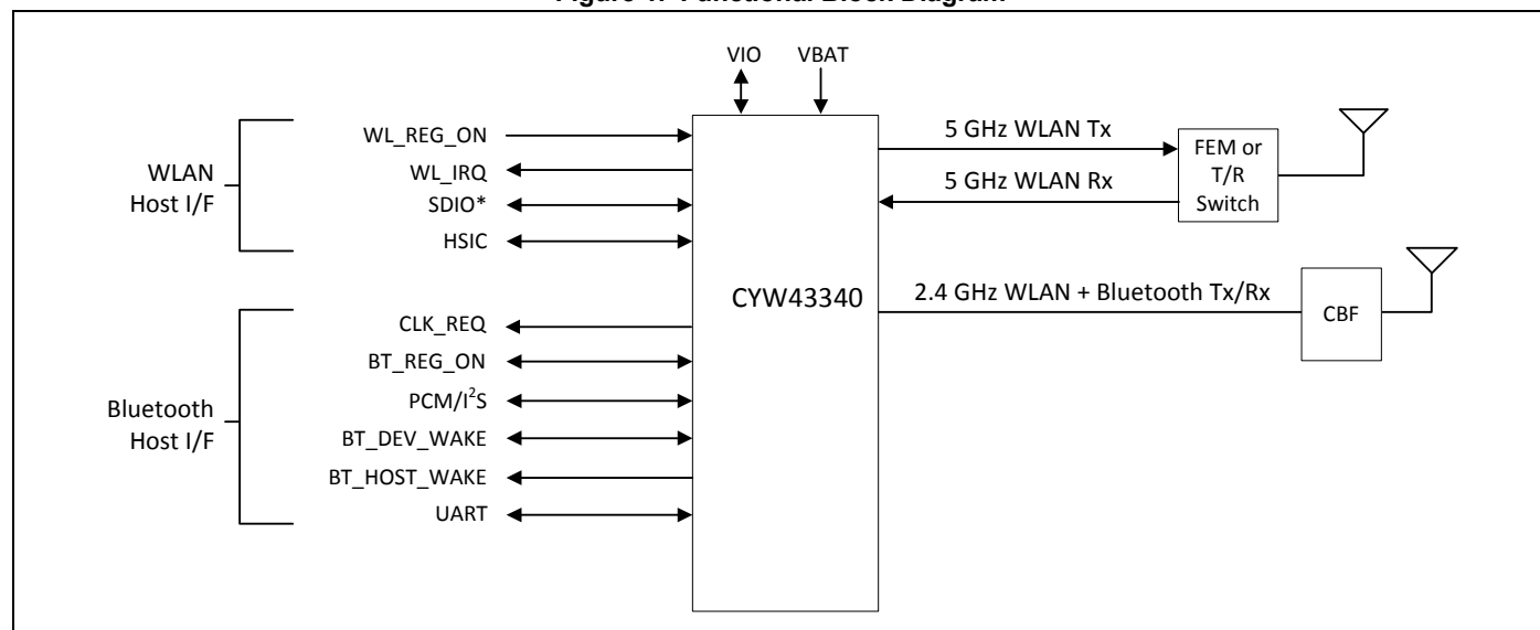
Figure 1. Functional Block Diagram
