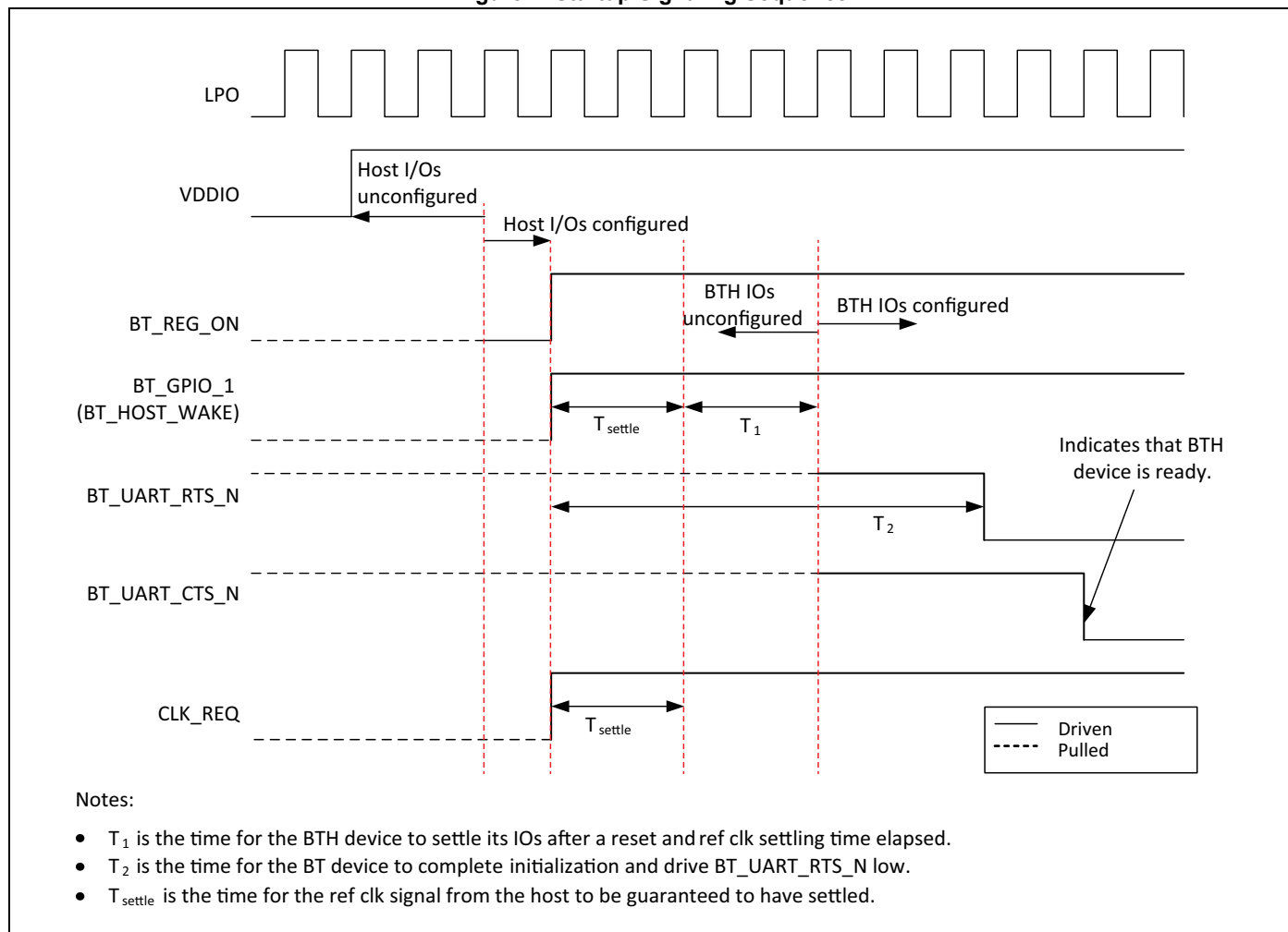
Figure 7. Startup Signaling Sequence
