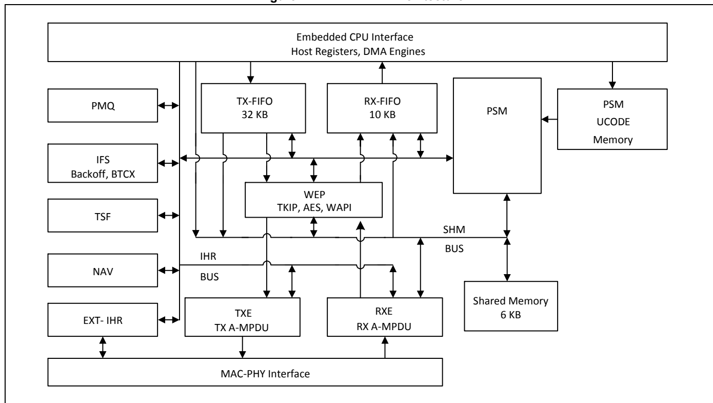
Figure 24. WLAN MAC Architecture
