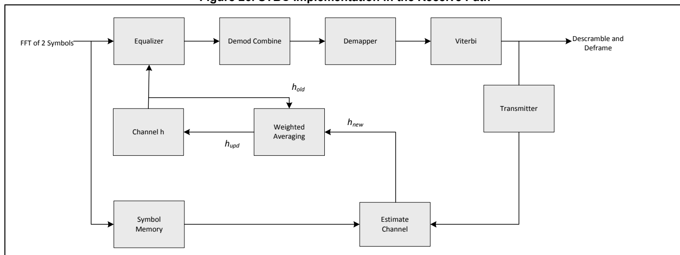
Figure 26. STBC Implementation in the Receive Path
