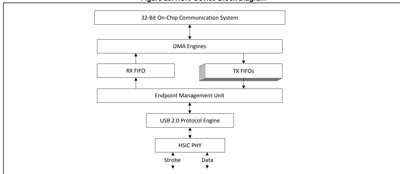
Figure 23. HSIC Device Block Diagram
