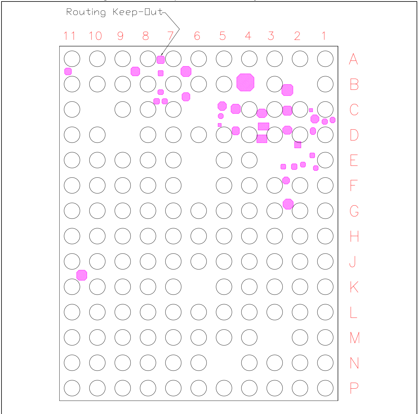
Figure 38. WLPGA Keep-Out Areas for PCB Layout—Bottom View
