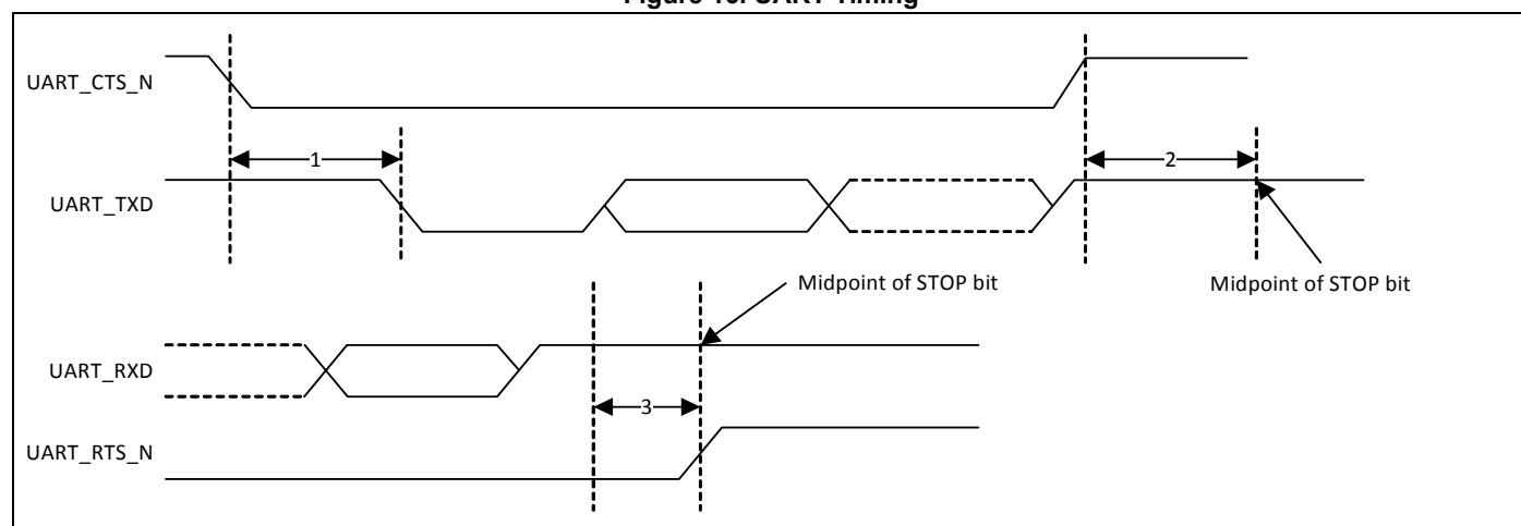
Figure 16. UART Timing
