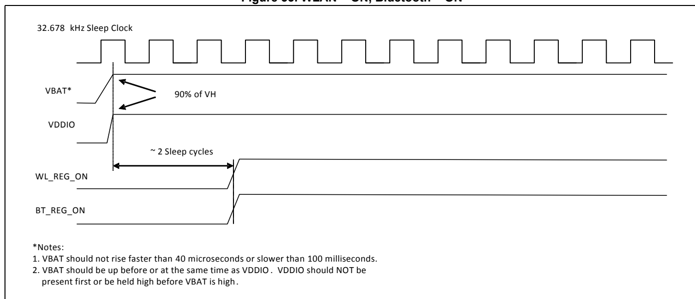
Figure 33. WLAN = ON, Bluetooth = ON
