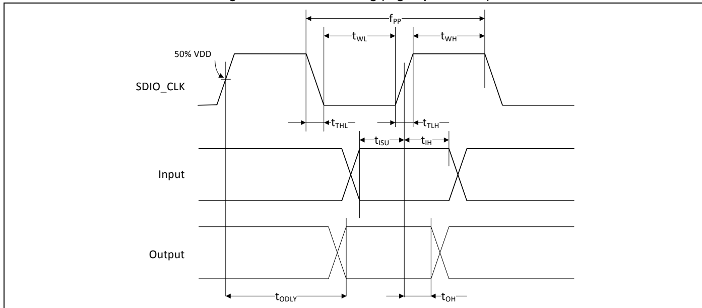
Figure 32. SDIO Bus Timing (High-Speed Mode)
