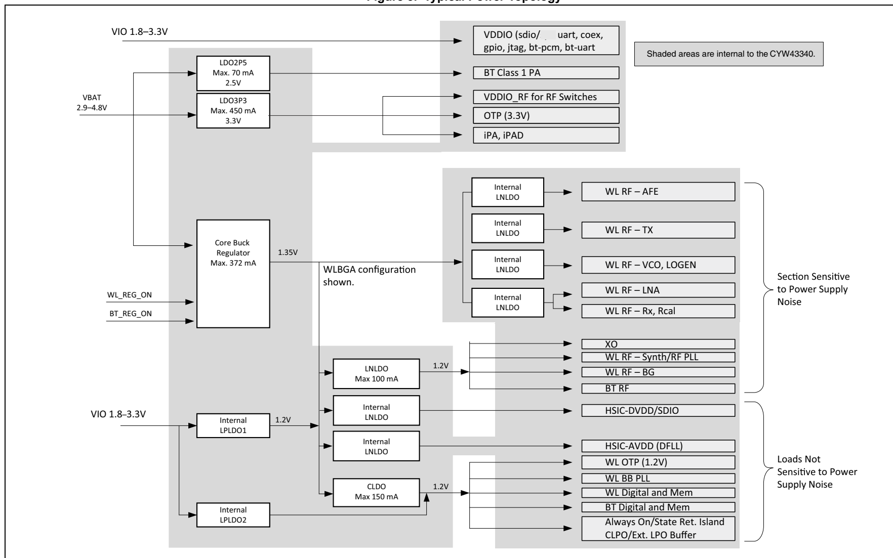
Figure 3. Typical Power Topology
