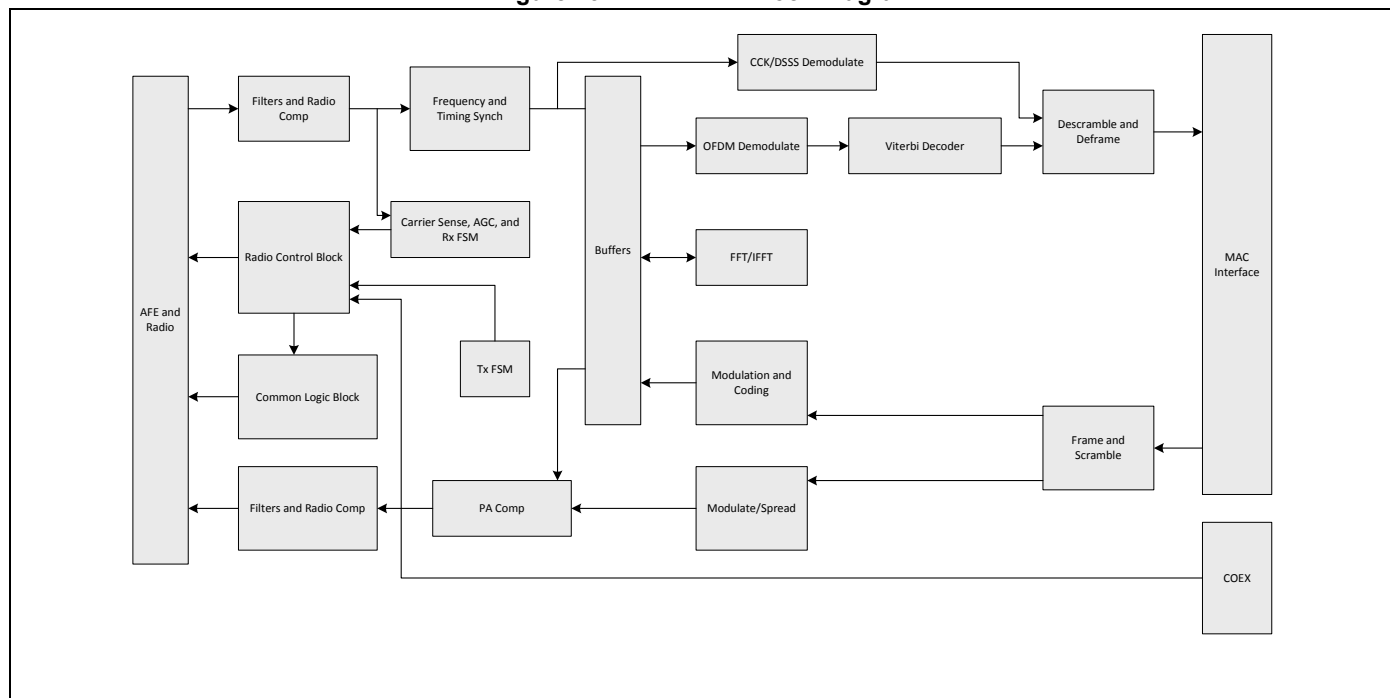
Figure 25. WLAN PHY Block Diagram
