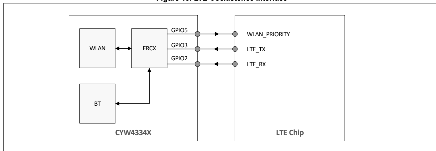
Figure 19. LTE Coexistence Interface
