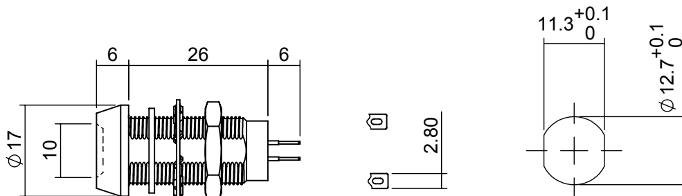
Mounting Hole
