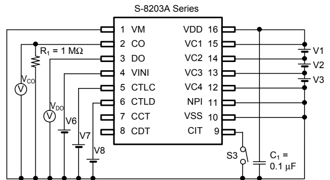
Figure 5 Test Circuit 2
