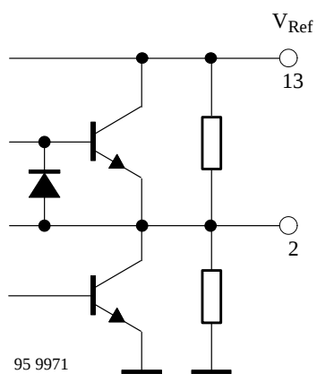
Figure 5. Pin 2 OP_{out}
