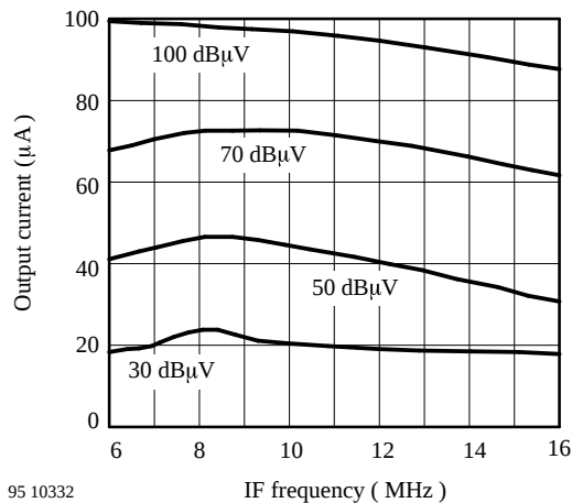
Figure 21. IF-frequency response
