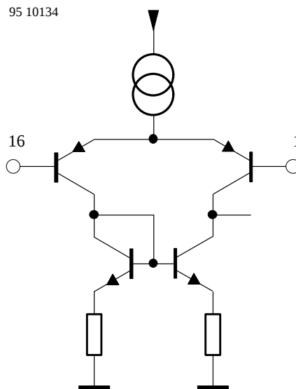
Figure 19. Pin 16 OP_{in-}
