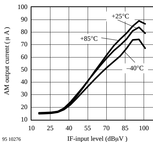
Figure 25. AM-demodulator characteristic vs. temperature
