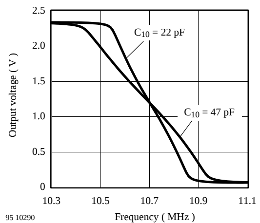
Figure 28. FM-discriminator characteristic
