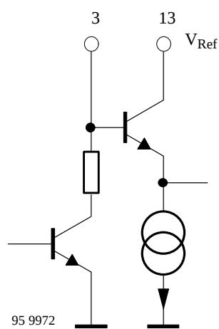
Figure 6. Pin 3 RC_{wake}
