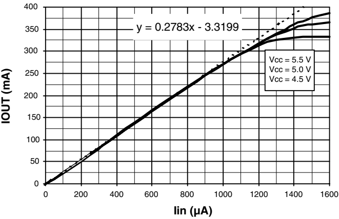
Figure 8. Voltage Compliance R ( I_{OUT} to V_{CC} ) = 5.9 Ω
