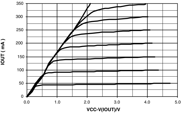
Figure 8. Voltage Compliance R ( I_{OUT} to V_{CC} ) = 5.9 Ω
