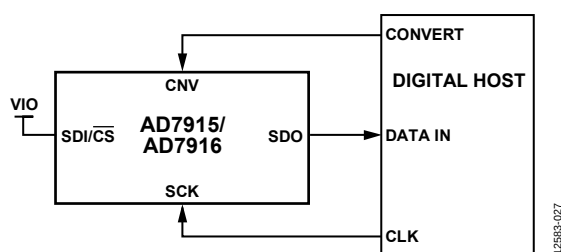
Figure 35. \overline{CS} Mode Without Busy Indicator, 3-Wire Connection Diagram (SDI High)
