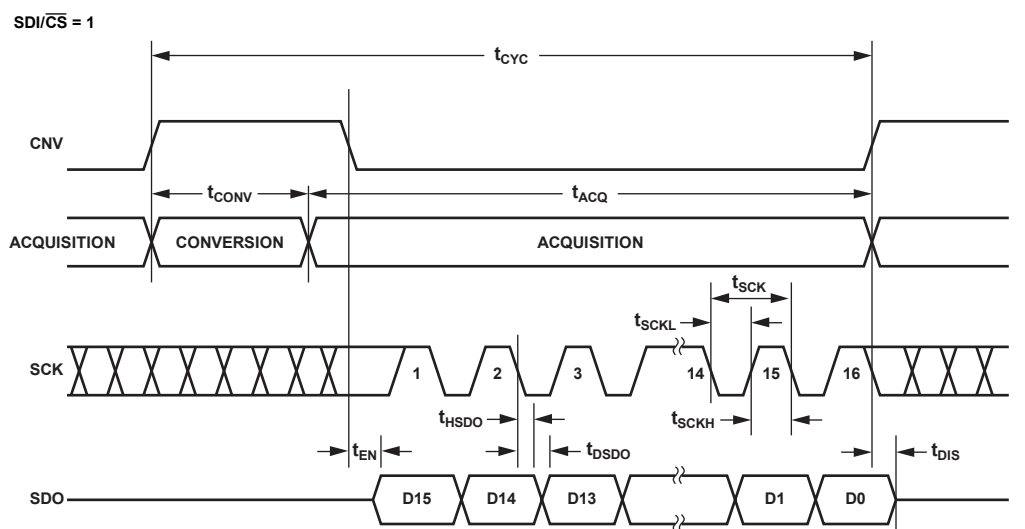
Figure 36. \overline{CS} Mode Without Busy Indicator, 3-Wire Serial Interface Timing (SDI High)
