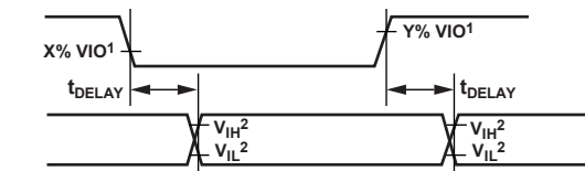
1 FOR V_{IO} \leq 3.0\text{ V} , X = 90 AND Y = 10 ; FOR V_{IO} > 3.0\text{ V} , X = 70 AND Y = 30 . 2 MINIMUM V_{IH} AND MAXIMUM V_{IL} USED. SEE THE DIGITAL INPUTS SPECIFICATIONS IN TABLE 3.
