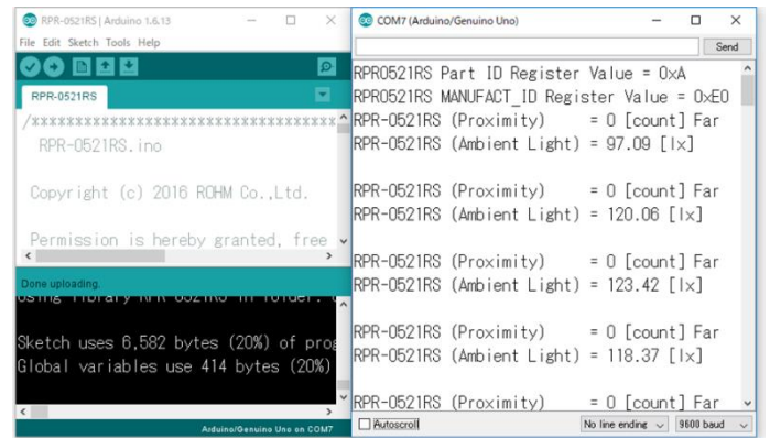
Figure 6. Serial Monitor
