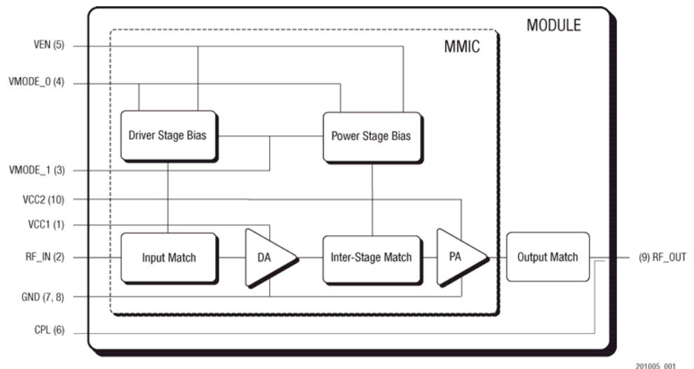
Figure 1. SKY77198-12 Functional Block Diagram
