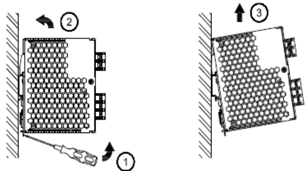
Fig. 2.2 Dismounting
