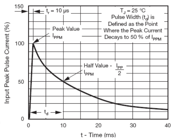
Fig.2 Pulse Waveform
