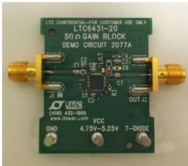
Figure 3. Demo Board
