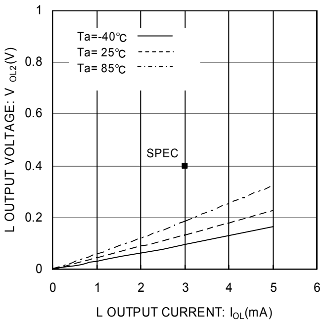
Fig. 6 'L' output voltage V_{OL1}(V_{CC}=2.5V)
