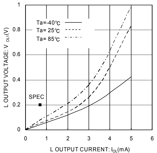
Fig.7 'L' output voltage V_{OL2}(V_{CC}=1.7V)
