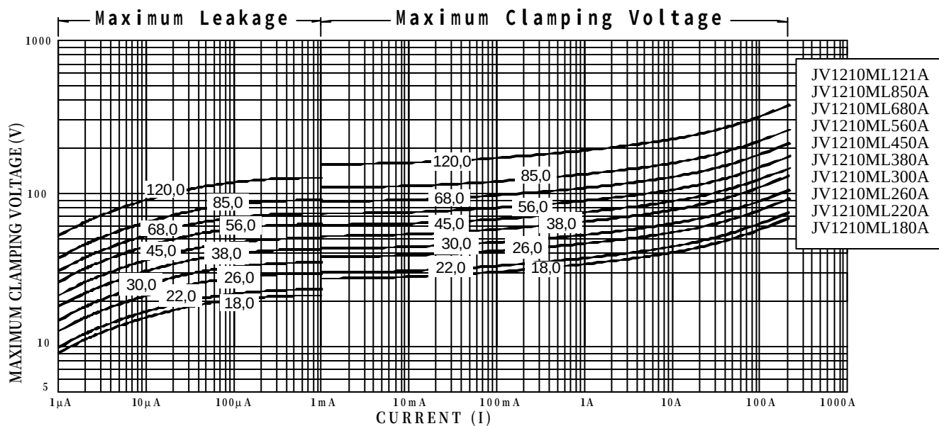
V/I Characteristics
