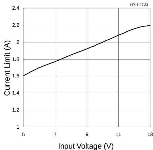
Current Limit vs. Input Voltage
