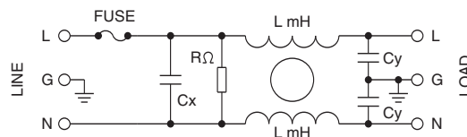
CIRCUIT DIAGRAM
