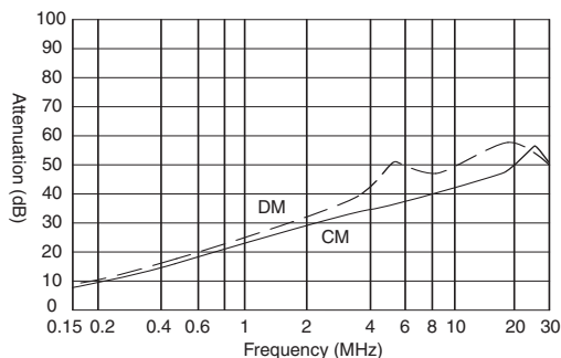
PLF-10DZ2R
