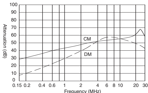
PLF-10DZ2R
