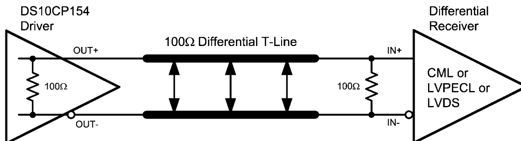
Typical DS10CP154A Output DC-Coupled Interface to an LVDS, CML or LVPECL Receiver
