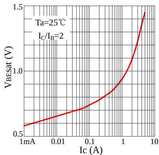
Fig4 V_{BEsat} - I_C
