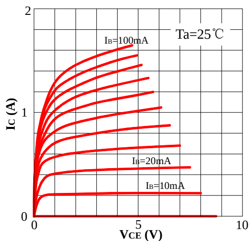
Fig1 Static Characteristic
