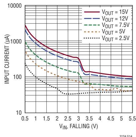
Burst Mode No-Load Input Current vs V_{IN}
