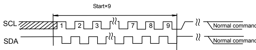
Fig.39-(c) START × 9 + command input
