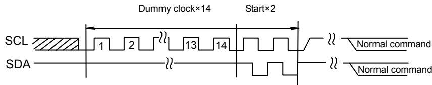
Fig.39-(a) The case of 14 Dummy clock + START + START+ command input
