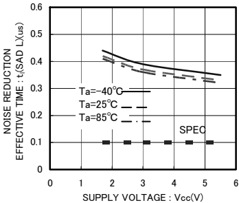
Fig.29 Noise reduction effective time t_i(\text{SDA L})
