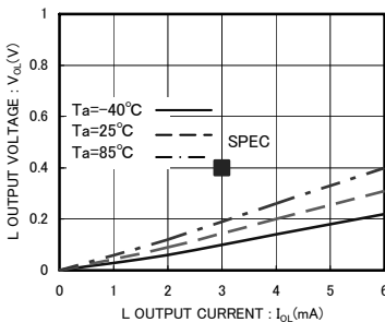
Fig.7 'L' output voltage V_{OL}-I_{OL} ( V_{CC}=2.5V )
