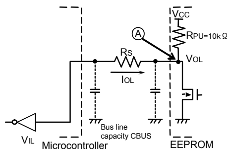
Fig.45 I/O circuit diagram
