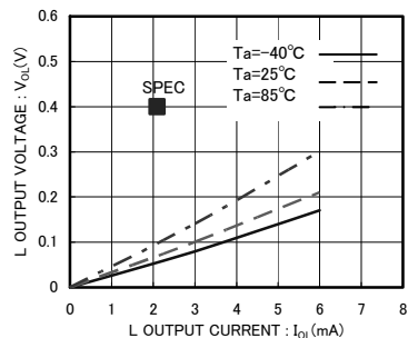
Fig.6 'L' output voltage V_{OL}-I_{OL} ( V_{CC}=1.7V )
