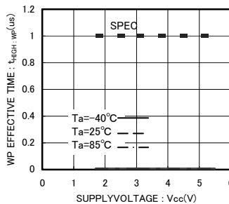
Fig.31 WP effective time t_{HGH : WP}
