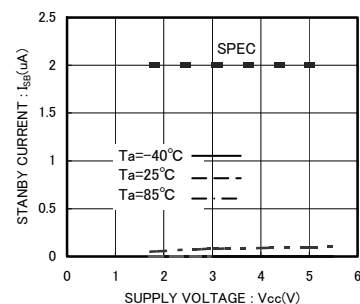
Fig.12 Standby operation I_{SB}
