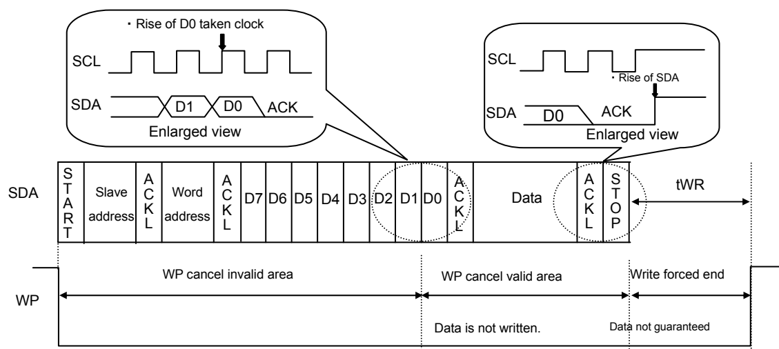
Fig.41 WP valid timing
