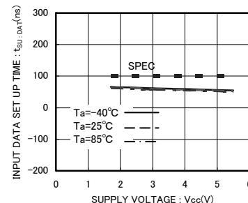
Fig.21 Input Data setup time t_{SU:DAT(LOW)}
