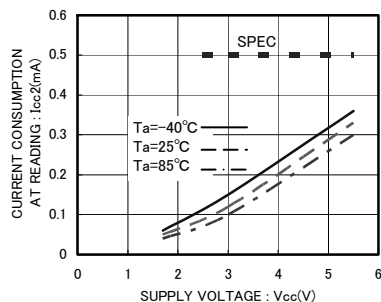
Fig.11 Current consumption at READ operation I_{CC2} ( f_{sc1}=400\text{kHz} )
