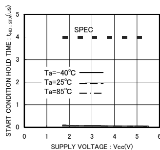
Fig.16 Start Condition Hold Time t_{HD:STA}
