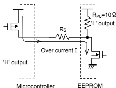
Fig.46 I/O circuit diagram
