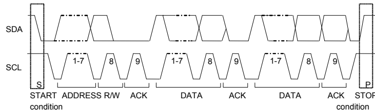
Fig.32 Data transfer timing
