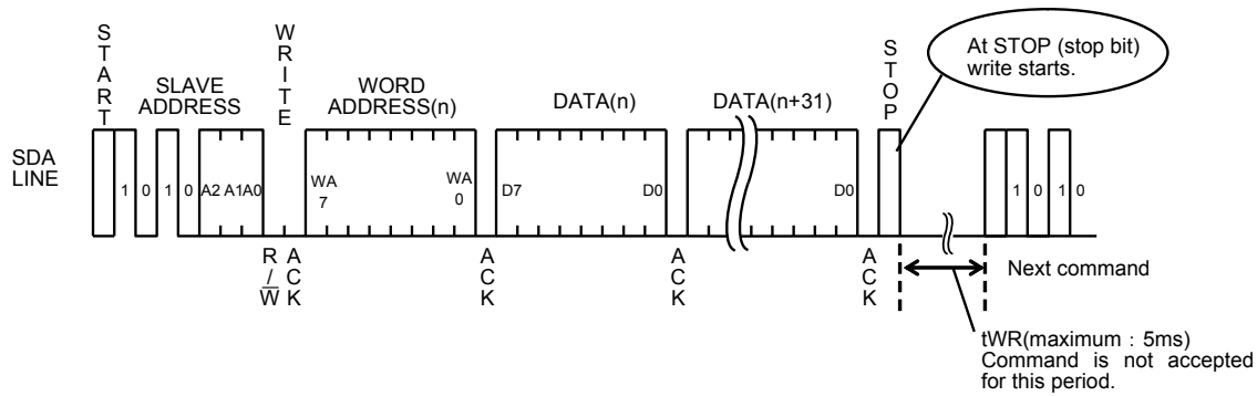
Fig.35 Page write cycle
