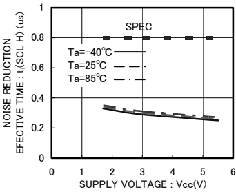
Fig.26 Noise reduction effective time t_i(\text{SCL H})
