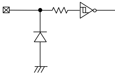
Fig.47 Input pin circuit diagram
