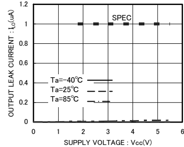
Fig.9 Output leak current I_{LO} (SDA)
