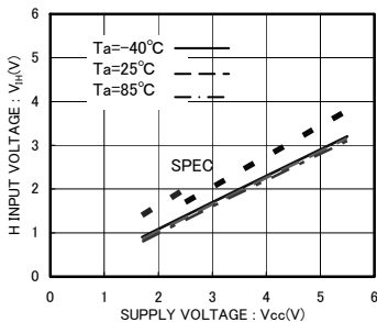
Fig.4 'H' input voltage V_{IH} (A0,A1,A2,SCL,SDA,WP)
