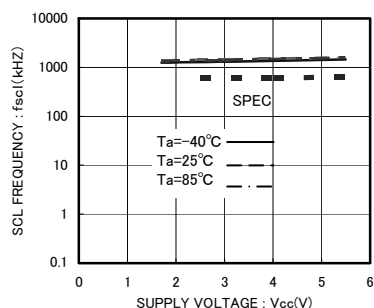
Fig.13 SCL frequency f_{sc1}
