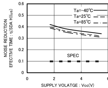
Fig.28 Noise reduction effective time t_i(\text{SDA H})
