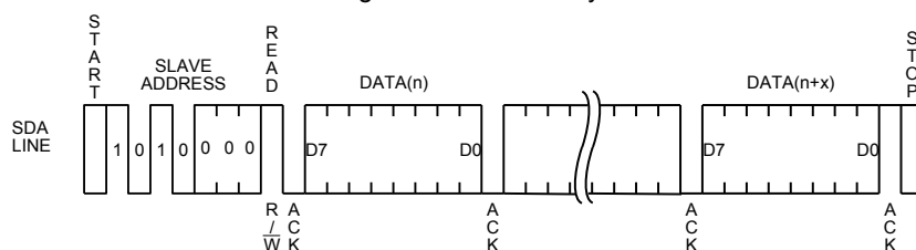
Fig.37 Current read cycle
