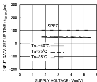
Fig.20 Input Data Setup Time t_{SU:DAT(HIGH)}
