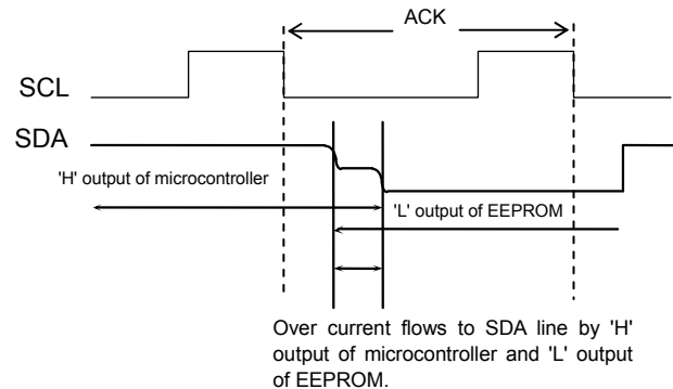
Fig.44 Input/output collision timing
