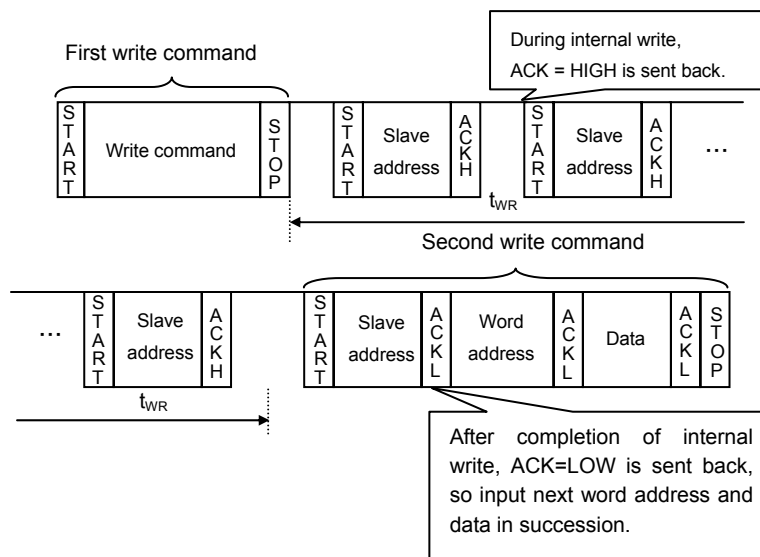
Fig.40 Case to continuously write by acknowledge polling
