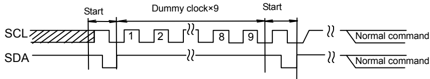
Fig.39-(b) The case of START+9 Dummy clock + START + command input
