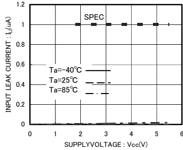
Fig.8 Input leak current I_{LI} (A0,A1,A2,SCL,WP)
