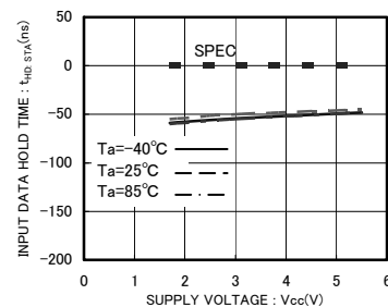
Fig.18 Input Data Hold Time t_{HD:DAT(HIGH)}
