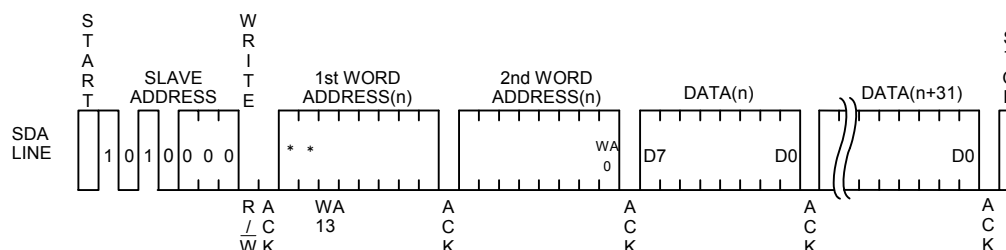
Fig.34 Page write cycle
