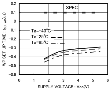
Fig.30 WP setup time t_{SU : WP}
