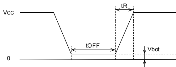
Fig.49 Rise waveform diagram
