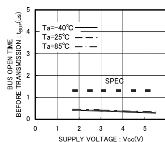
Fig.24 BUS open time before transmission t_{BUF}
