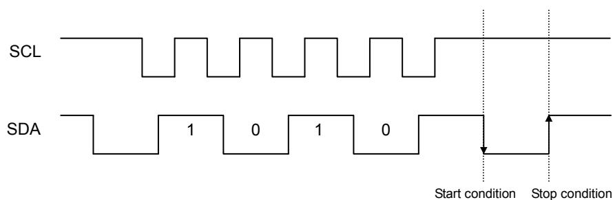
Fig.42 Case of cancel by start, stop condition during slave address input
