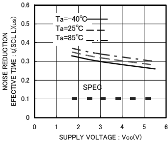
Fig.27 Noise reduction effective time t_i(\text{SCL L})
