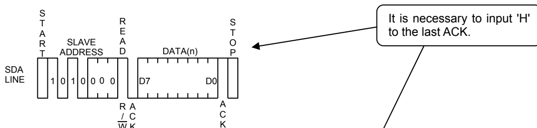
Fig.37 Current read cycle
