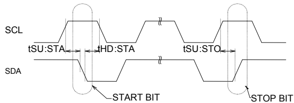
Fig.1-(b) Start - stop bit timing
