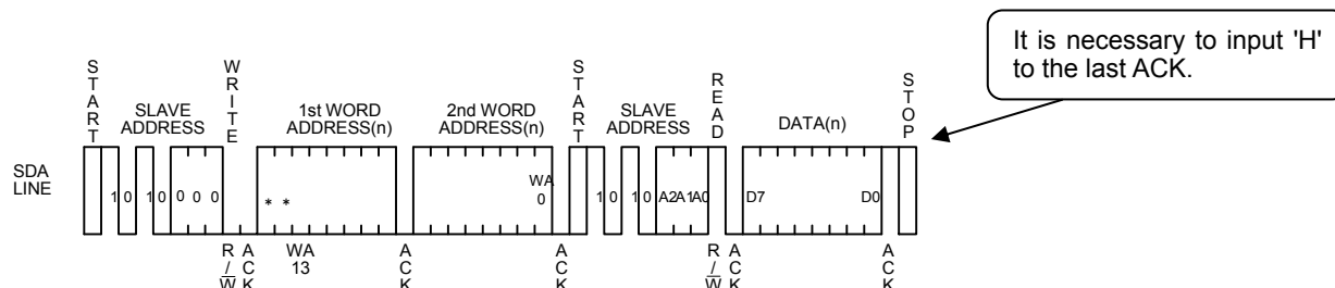
Fig.36 Random read cycle
