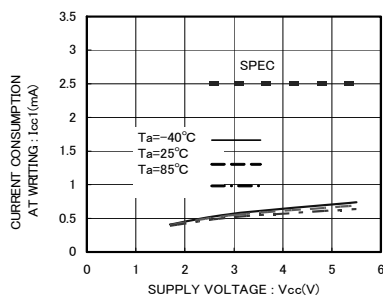
Fig.10 Current consumption at WRITE operation I_{CC1} ( f_{sc1}=400\text{kHz} )
