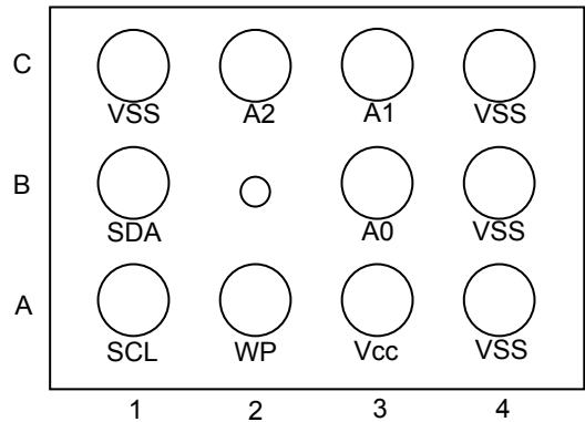
Fig.3 BU9897GUL-W(bottom view)
