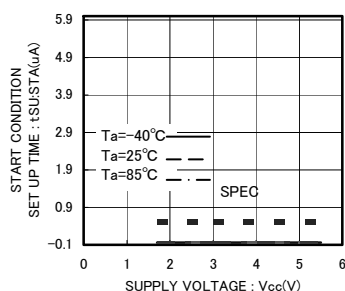
Fig.17 Start Condition Setup Time t_{SU:STA}
