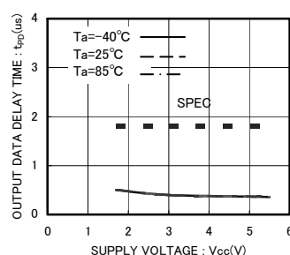
Fig.22 'L' Data output delay time t_{PO0}
