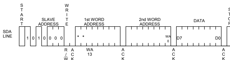
Fig.33 Byte write cycle
