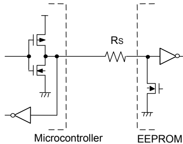
Fig.43 I/O circuit diagram
