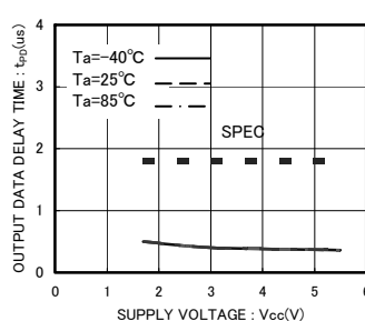
Fig.23 'H' Data output delay time t_{PO1}
