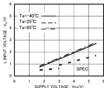
Fig.5 'L' input voltage V_{IL} (A0,A1,A2,SCL,SDA,WP)
