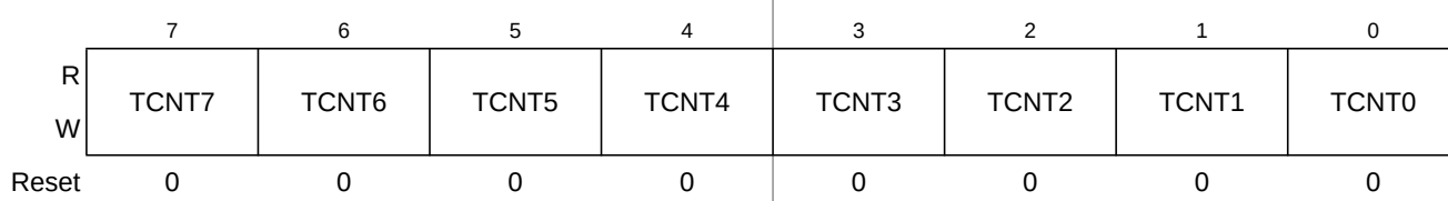
Figure 14-11. Timer Count Register Low (TCNTL)
