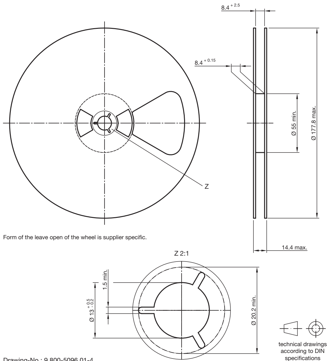
Fig. 11 - 7" Reel, 3000 Pieces
