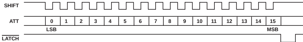
Figure 3. Control-Data-Input Timing
