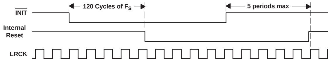
Figure 1. Reset Timing Relationships
